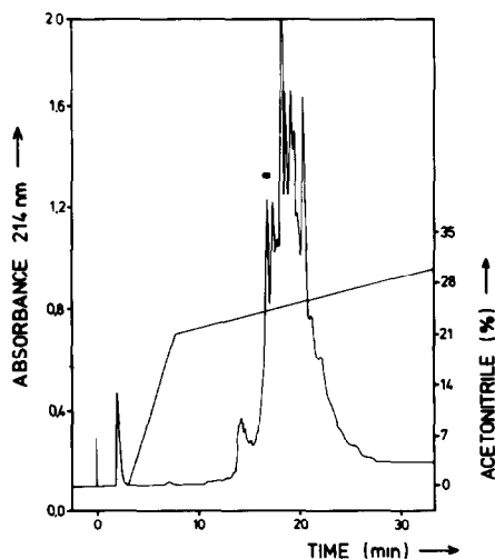
Fig.3. Reverse-phase HPLC of partially purified guinea pig neurotensin on a Supelcosil LC-3DP column. The peak with neurotensin-like immunoreactivity is indicated by the bar. (—) Concentration of acetonitrile in the elution solvent.
